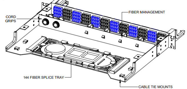
PANEL REAR (TOP REMOVED)
